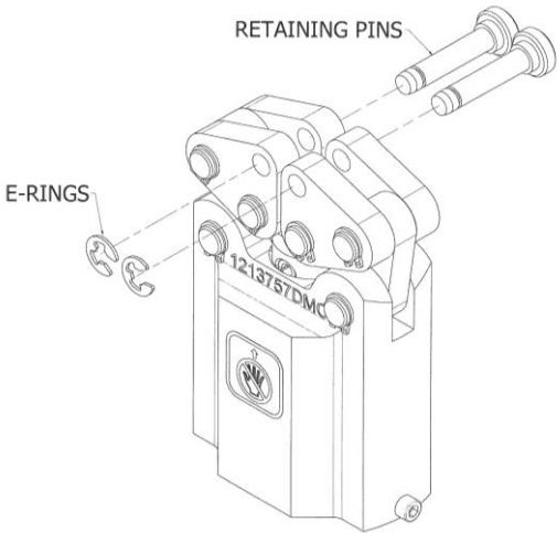
Figure 1. Remove Retaining Pins
